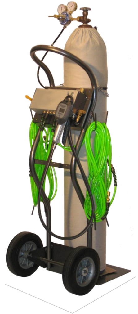
HC100 Portable Nitrogen Machine (Regulator & cylinder not included)
